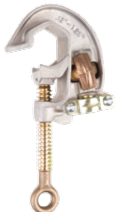
C6002275 Aluminum body, Smooth jaws, Bronze eyescrew with Acme threads, Bronze pressure-type terminals
