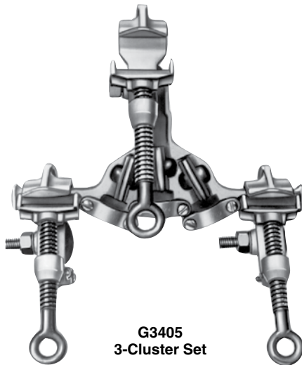
G3405 3-Cluster Set with C-Type Aluminum-body clamps,
