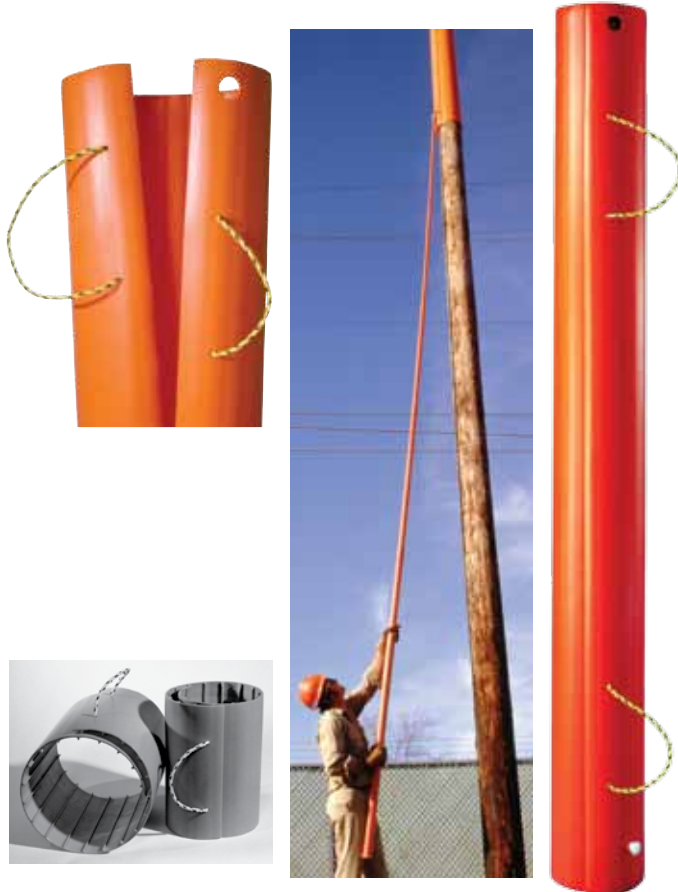
Pole covers can be removed easily from ground level using Chance telescoping tools.
