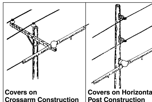
Deadend Cover couples with Conductor Cover
